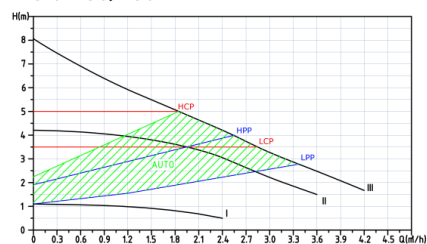
IVO 32-80/180
