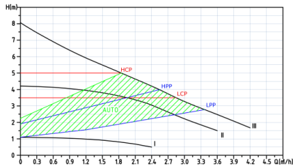
IVO 25-80/180
