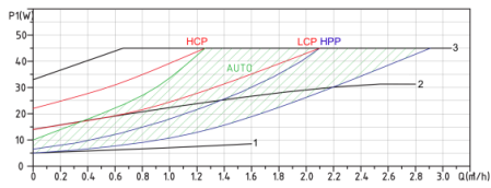
IVO 32-80/180
