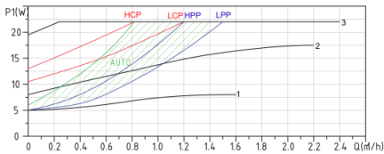
IVO 25-80/180
