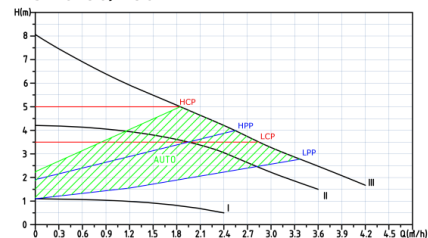
IVO 25-80/180
