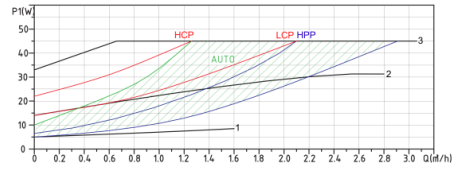
IVO 32-80/180
